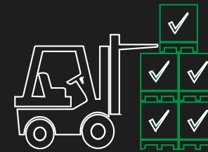
Logistic
